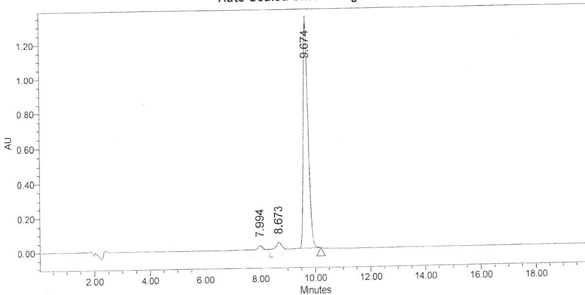
Auto-Scaled Chromatogram
